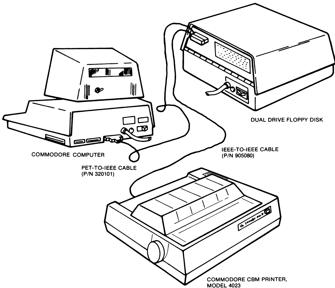
Figure 4. Multiple Hookup
