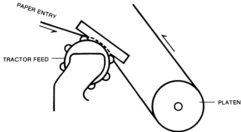
Figure 5. Paper Path
